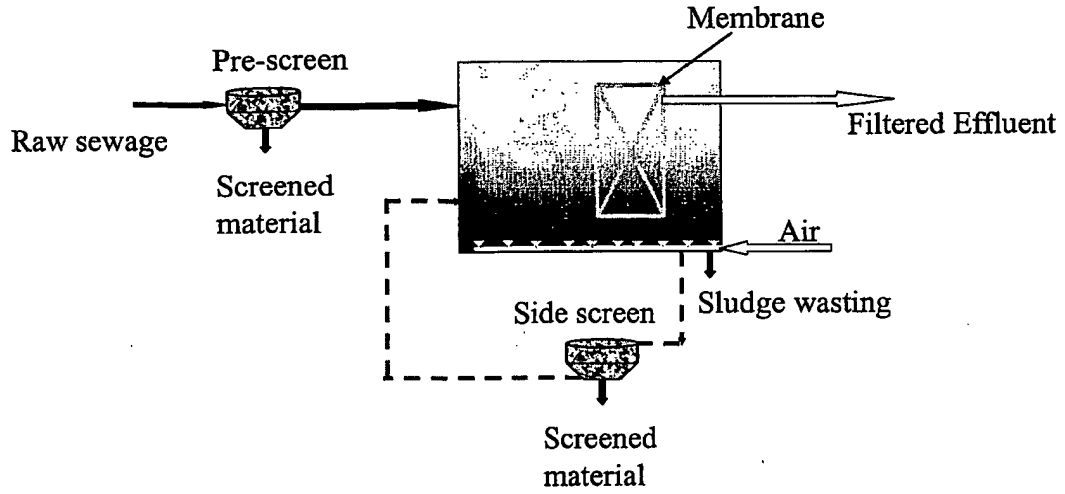
Figure 21 - Conventional MBR Configuration
